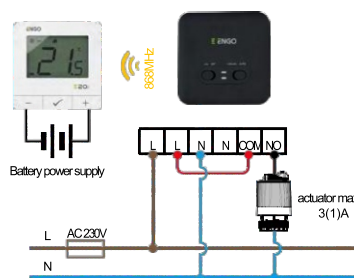
b) Connection diagrams for the actuator
