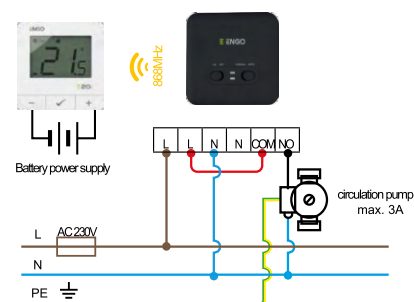
c) Connection diagrams for the circulation pump
