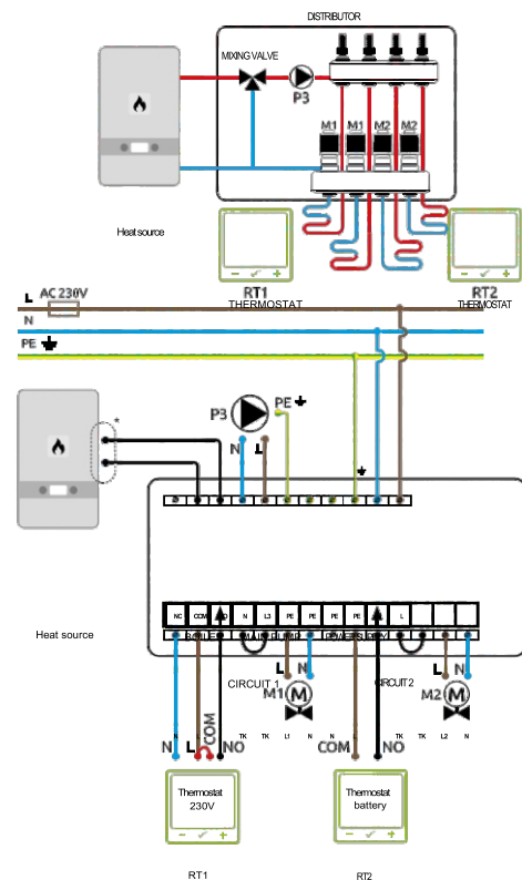
B) CONNECTING 2 HEATING ZONES OF UNDERFLOOR HEATING TO THE INTEGRATOR
